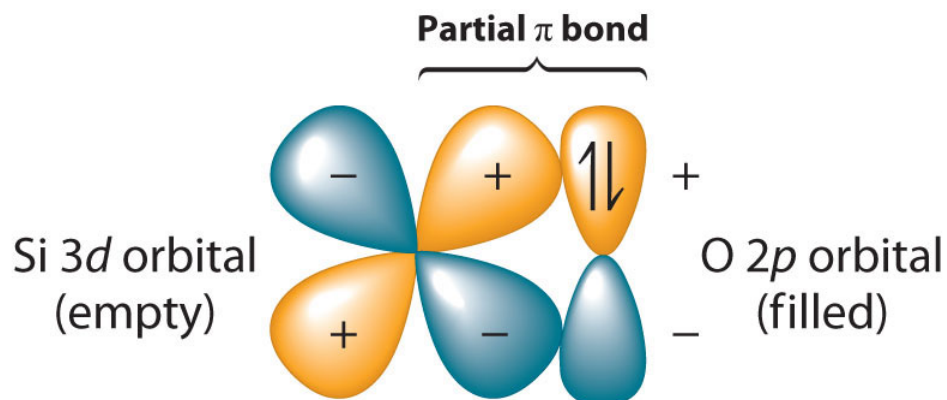
Figure 22.7 Pi Bonding between Silicon and Oxygen
