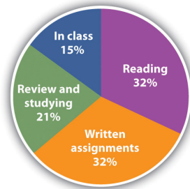
Figure 5.6 Pie Chart
