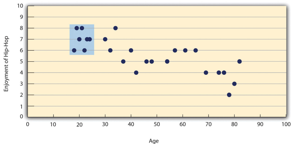
Figure 12.11 Hypothetical Data Showing How a Strong Overall Correlation Can Appear to Be Weak When One Variable Has a Restricted Range
