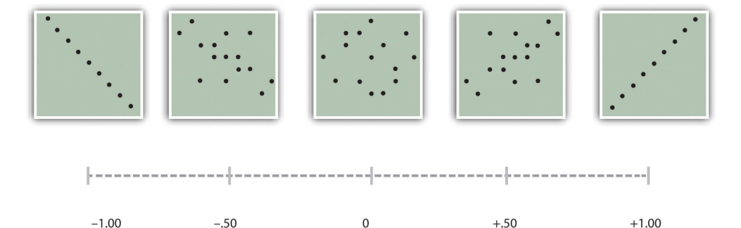
Figure 12.10 Pearson’s r Ranges From -1.00 (Representing the Strongest Possible Negative Relationship), Through 0 (Representing No Relationship), to +1.00 (Representing the Strongest Possible Positive Relationship)
