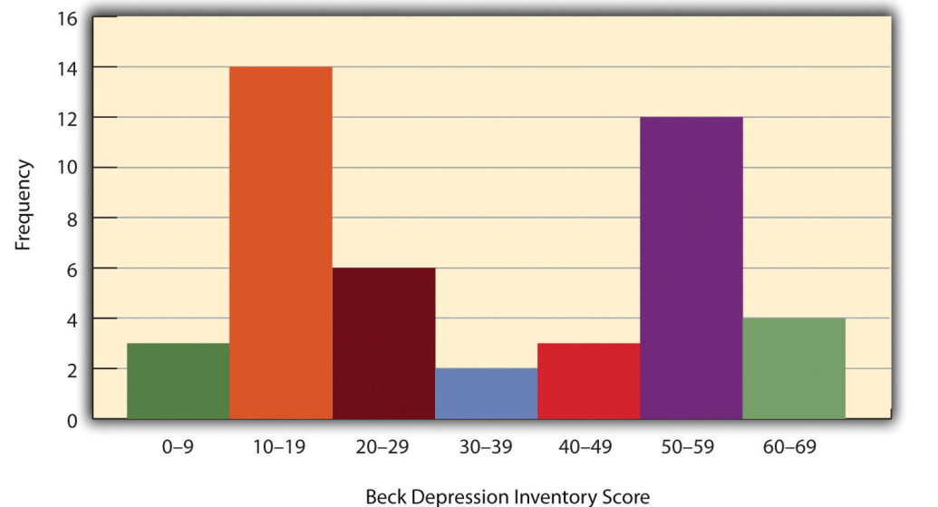
Figure 12.2 Histogram Showing a Hypothetical Bimodal Distribution of Scores on the Beck Depression Inventory
