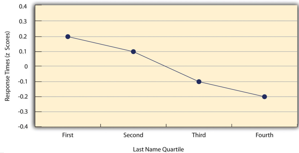
Figure 12.7 Line Graph Showing the Relationship Between the Alphabetical Position of People's Last Names and How Quickly Those People Respond to Offers of Consumer Goods
