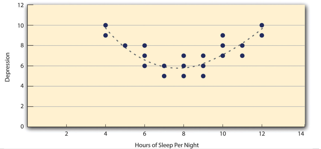
Figure 12.9 A Hypothetical Nonlinear Relationship Between How Much Sleep People Get per Night and How Depressed They Are
