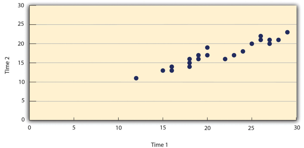
Figure 12.8 Statistical Relationship Between Several College Students' Scores on the Rosenberg Self-Esteem Scale Given on Two Occasions a Week Apart
