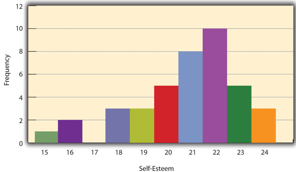
Figure 12.1 Histogram Showing the Distribution of Self-Esteem Scores Presented in Table 12.1 "Frequency Table Showing a Hypothetical Distribution of Scores on the Rosenberg Self-Esteem Scale"
