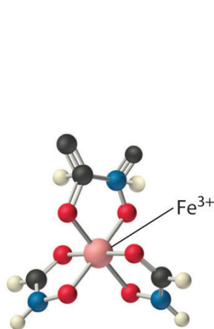
Fe(hydroxamate) 3
