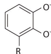
Catecholate ligand (2-)
