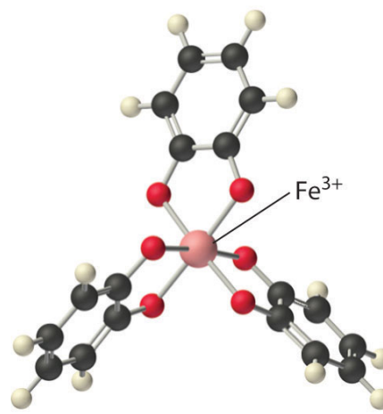
Fe(catecholate) 3 3-
