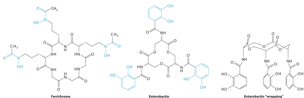
Figure 23.18 Siderophores
